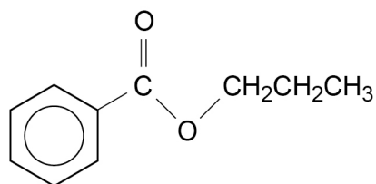
propyl benzoate
