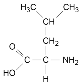
leucine
