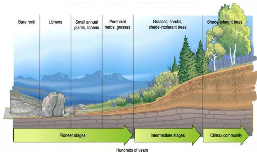
Lithosere succession
