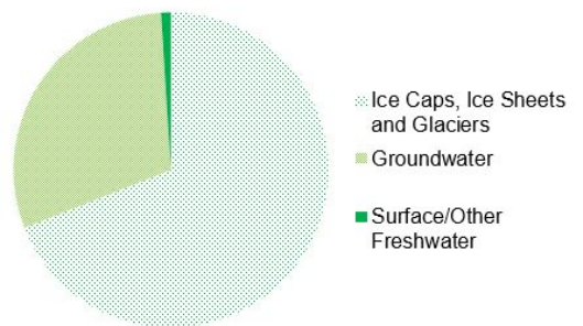
Freshwater
